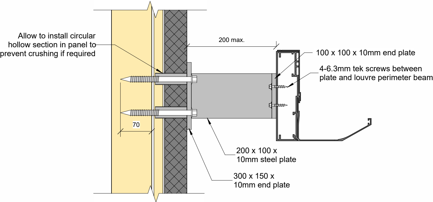
H BRACKET - NEW BUILDINGS ONLY 1 : 5
