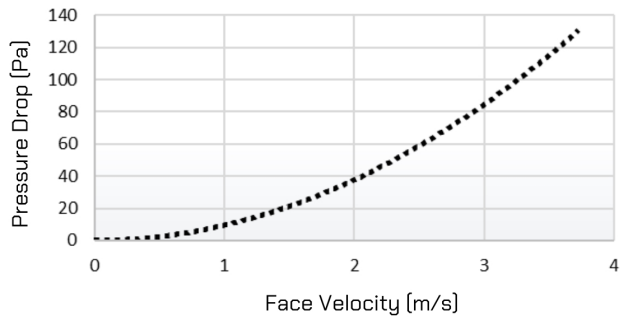
VL-50PL3 Pressure Drop
