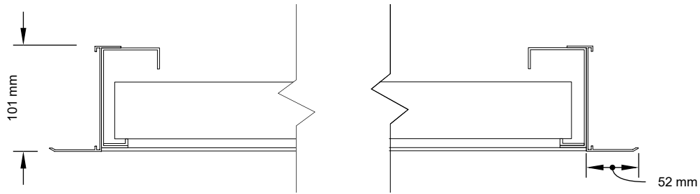
FLANGED FRAME - HORIZONTAL SECTION
