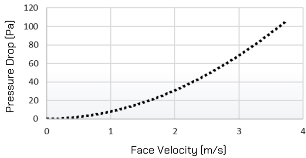
VL-50PL1 Pressure Drop
