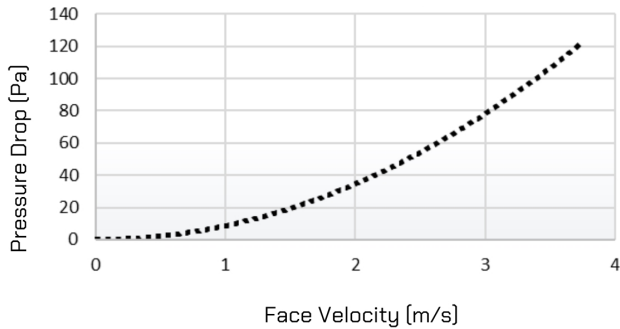
VL-50PL6 Pressure Drop
