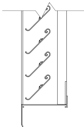
FLANGED FRAME VERTICAL SECTION
