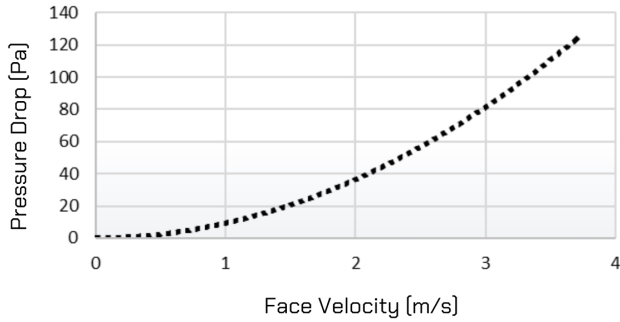
VL-50PL5 Pressure Drop
