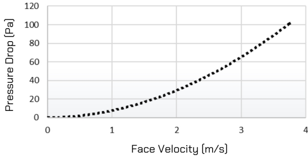
VL-50PL4 Pressure Drop
