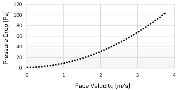
VL-50PL2 Pressure Drop
