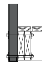
Side fixed to timber deck
