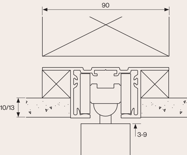
Full-Height Detail
