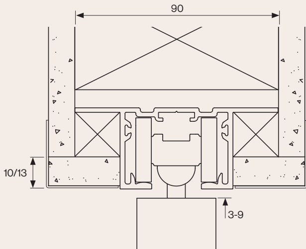
SquareStop Detail
