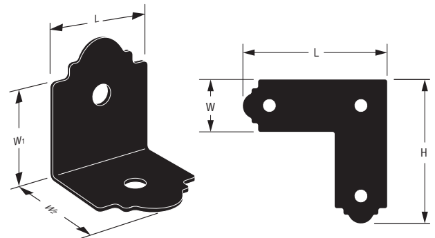
APA4 Heavy Angle
