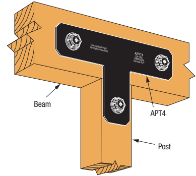
APT4 Post-to-Beam Corner Installation
