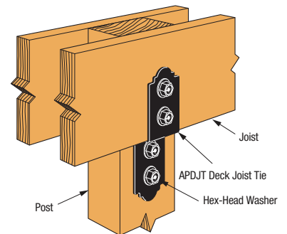
APDJT Joist-to-Post Connection
