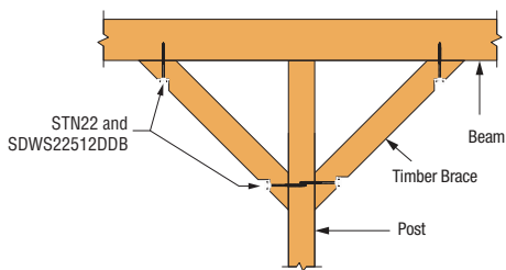
STN22 & SDWS Timber Brace
