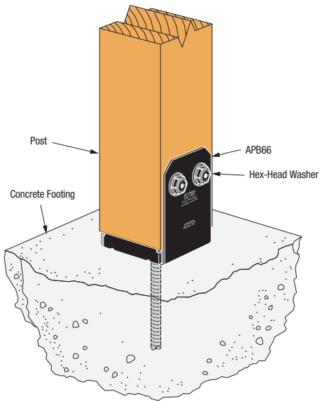
APB66 Post Base Installation
