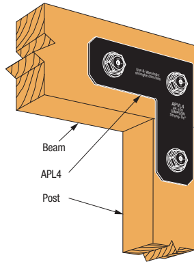
APL4 Post-to-Beam Corner Installation
