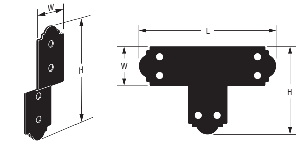
APDJT Deck Joist Tie
