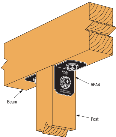
APA Post-to-Beam Corner Installation
