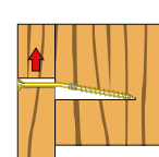
5: plastic hinge - timber 2
