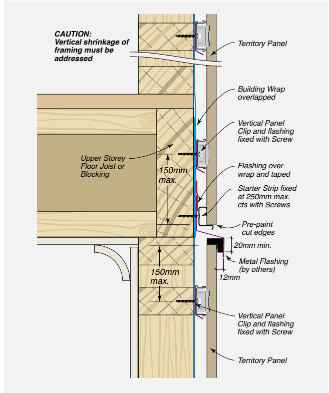
FIGURE 8.22 Horizontal Control Joint – Second Storey Junction – Closed Cavity
