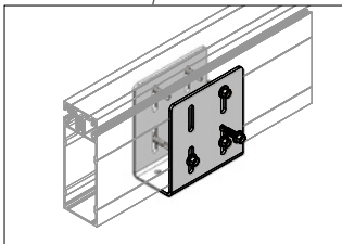
Saddle Brackets
