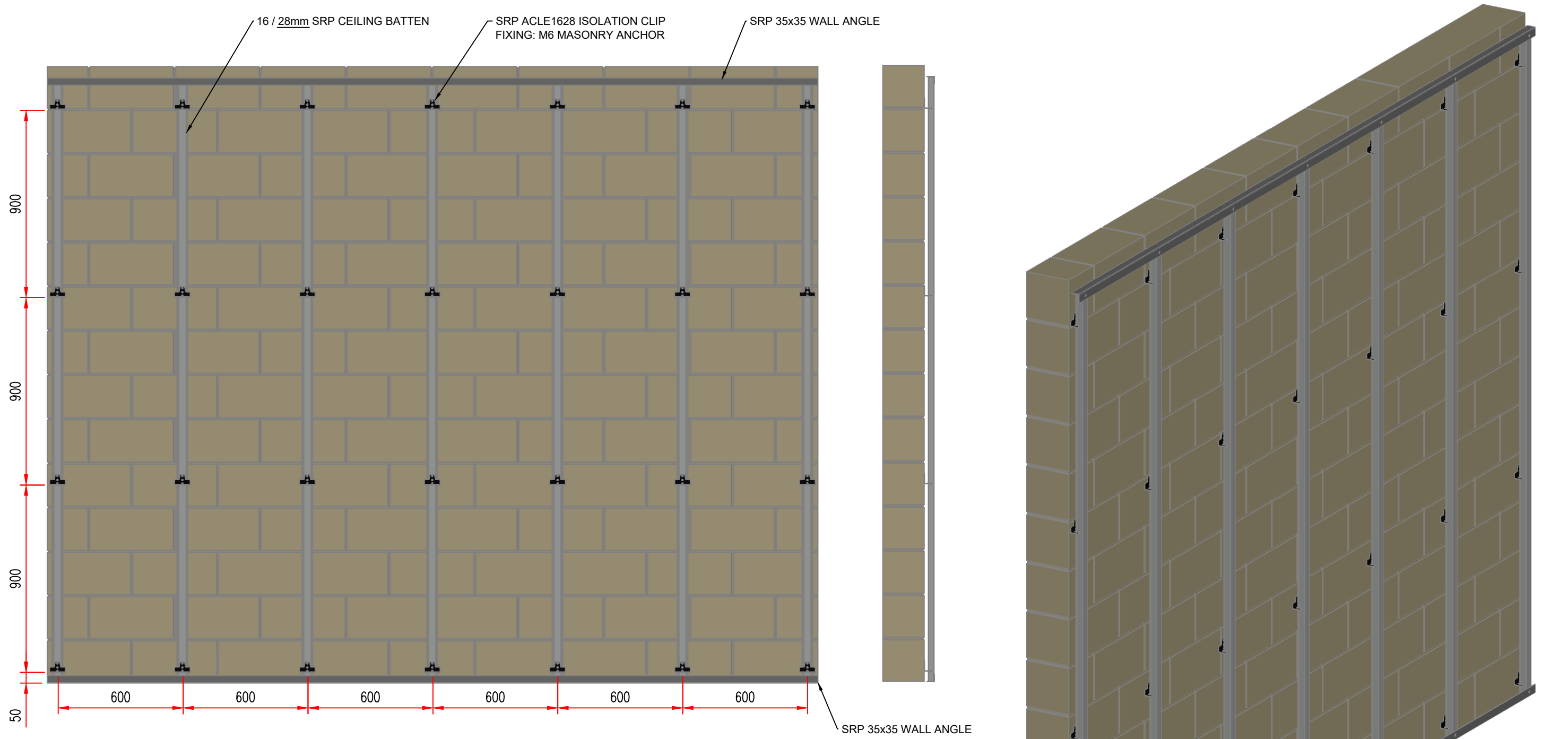
STANDARD SRP WALL STRAPPING SYSTEM 16/28 BATTEN WITH ADJUSTABLE WALL FIX CLIP + WALL ANGLE
