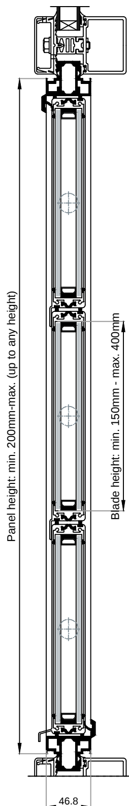
VERTICAL SECTION
