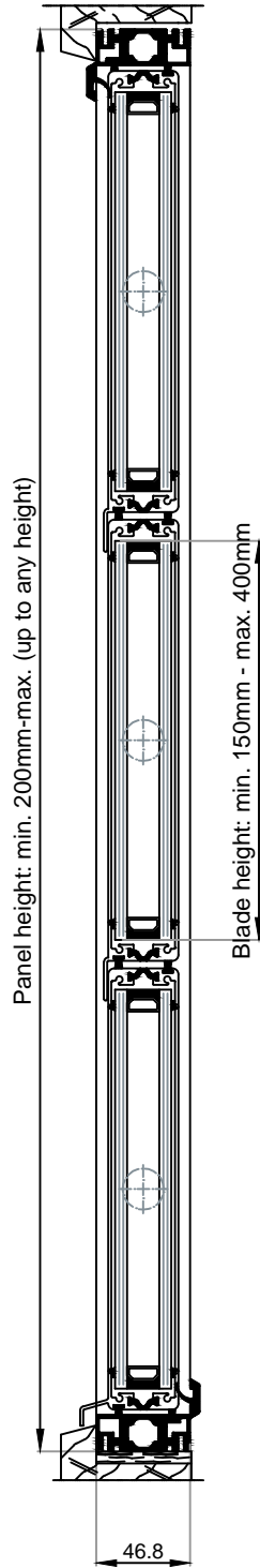
VERTICAL SECTION
