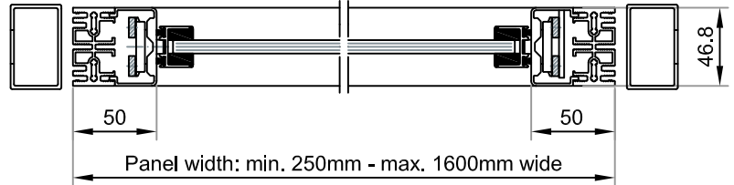
HORIZONTAL SECTION
