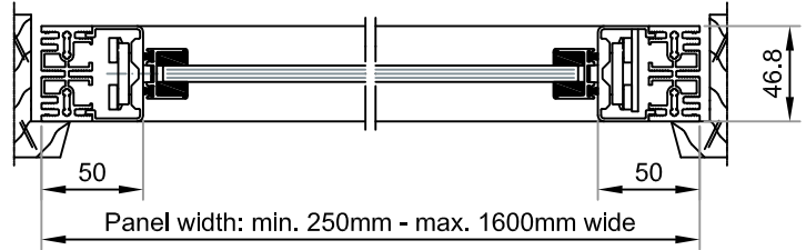
HORIZONTAL SECTION
