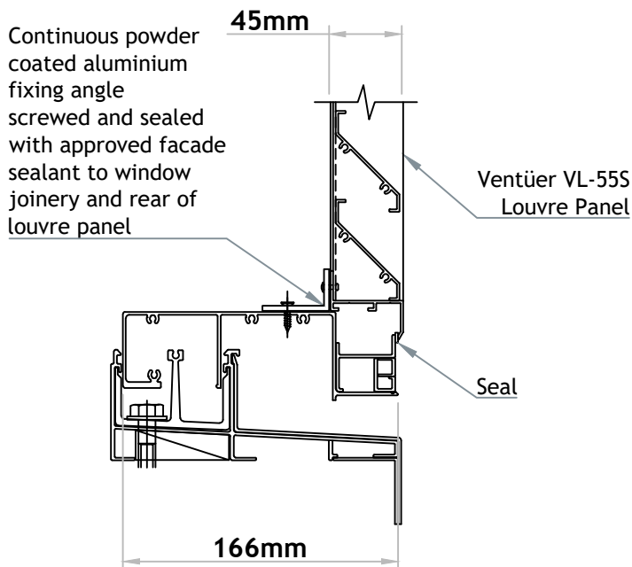
VL-55S (FLANGED FRAME) SILL DETAIL 03 SCALE 1 : 4
