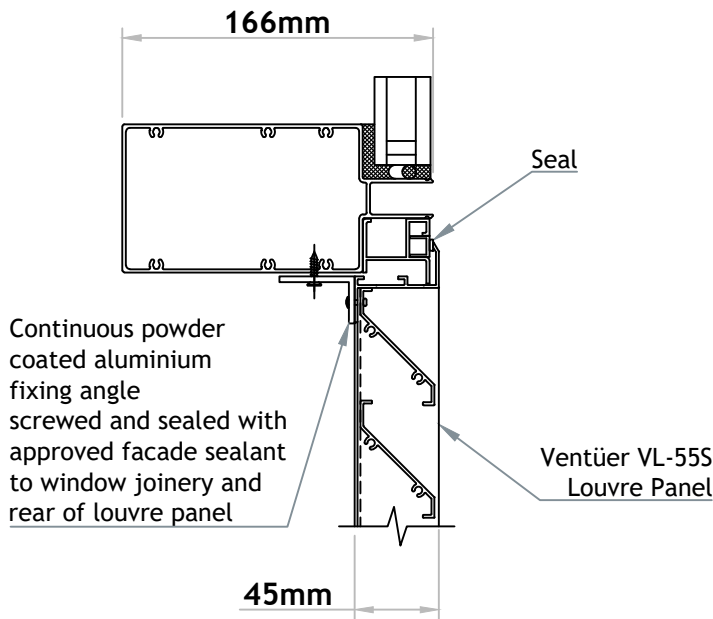
VL-55S (FLANGED FRAME) HEAD DETAIL 01 SCALE 1 : 4
