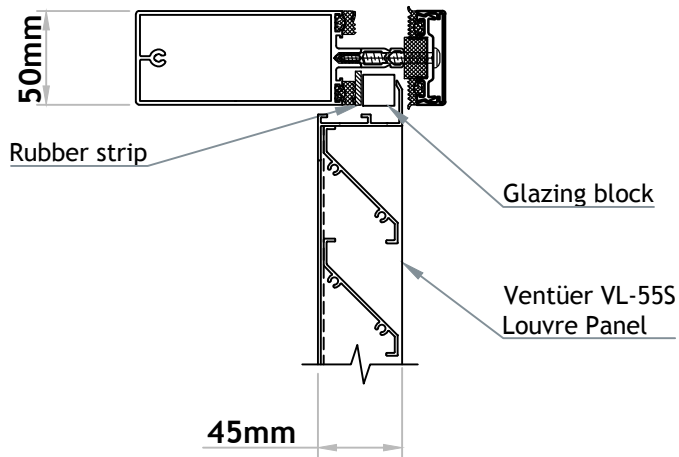
VL-55S (FLANGED FRAME) HEAD DETAIL 01 SCALE 1 : 4
