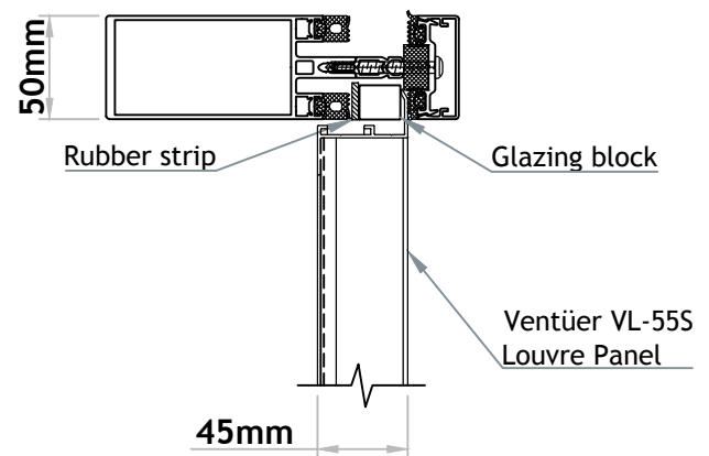
VL-55S (FLANGED FRAME) JAMB DETAIL 02 SCALE 1 : 4
