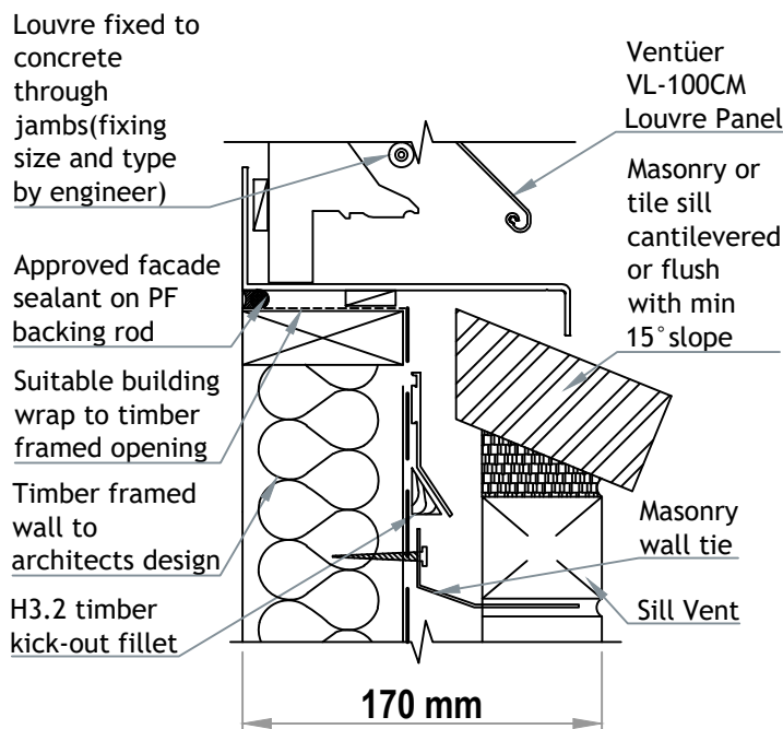
VL-100CM (FLANGED FRAME) SILL DETAIL 03 SCALE 1 : 4
