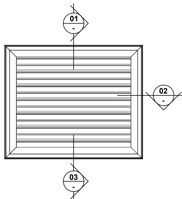
VL-100CM LOUVRE (FLANGED FRAME)
