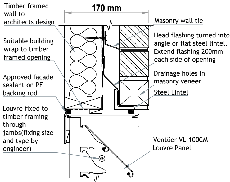
VL-100CM (FLANGED FRAME) HEAD DETAIL 01 SCALE 1 : 4
