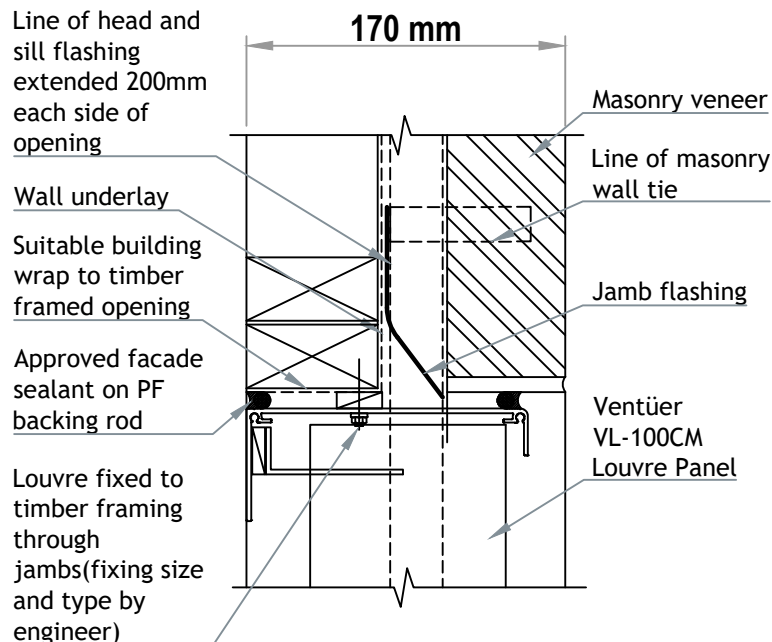
VL-100CM (FLANGED FRAME) JAMB DETAIL 02 SCALE 1 : 4
