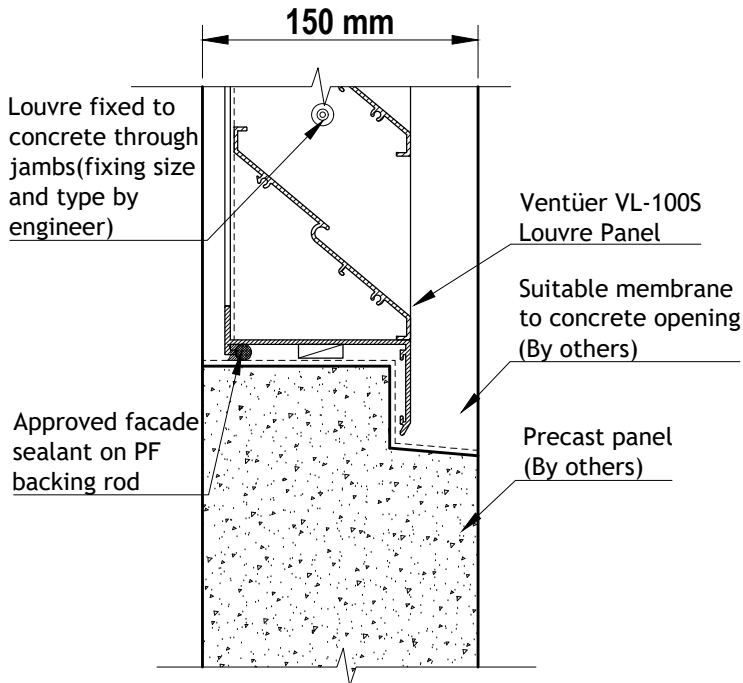
VL-100S (FLANGED FRAME) SILL DETAIL 03 SCALE 1 : 4
