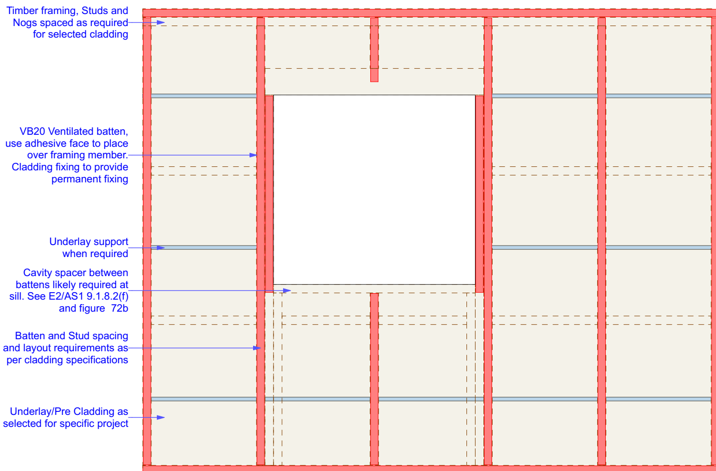
VB20 Ventilated Batten Horizontal Cladding layout
