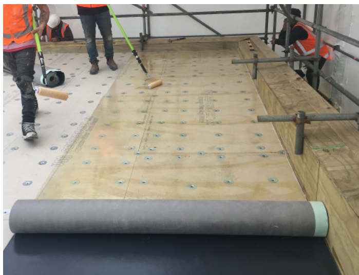
Rooflogic Fleeceback being installed over RL Roof Board HD and adhered with RL FTR 490u adhesive.
