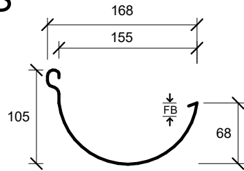
ROOFING INDUSTRIES 168mm HALF ROUND GUTTER
