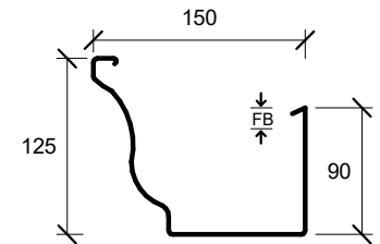
ROOFING INDUSTRIES 150mm OLD GOTHIC GUTTER
