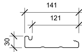
136 FASCIA COVER = 121mm
