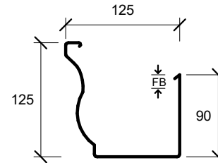
ROOFING INDUSTRIES 125mm OLD GOTHIC GUTTER
