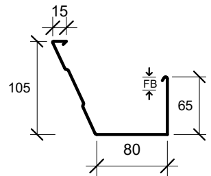
ROOFING INDUSTRIES J LINE GUTTER
