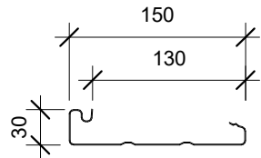
150 FASCIA COVER = 130mm
