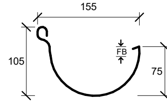
ROOFING INDUSTRIES 155mm HALF ROUND GUTTER
