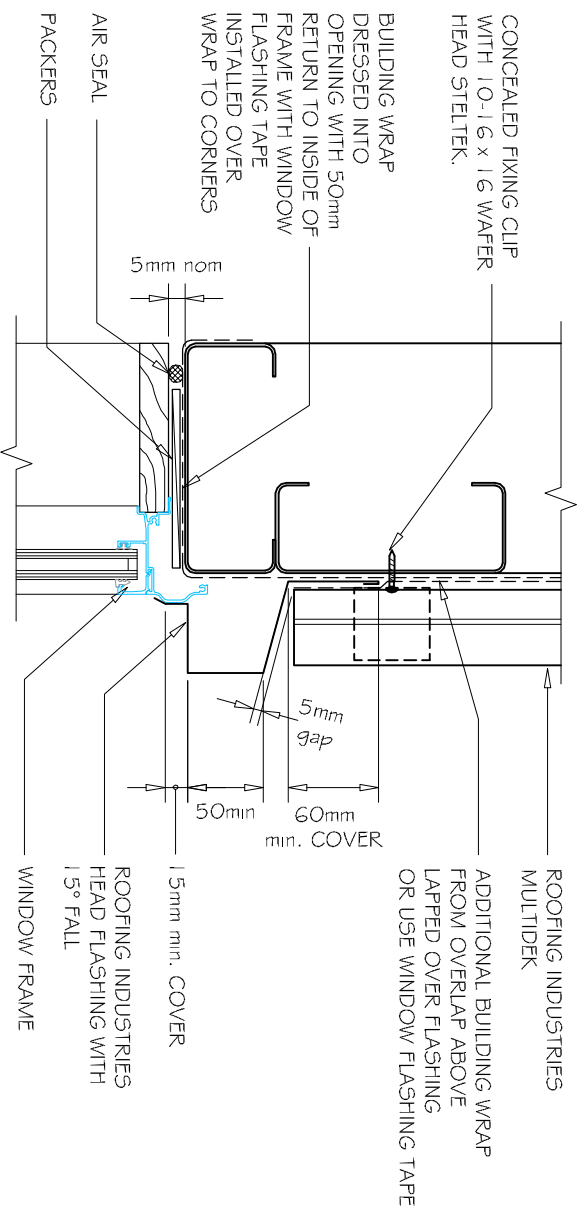
A WINDOW HEAD VERTICAL MULTIDEK 1:5
