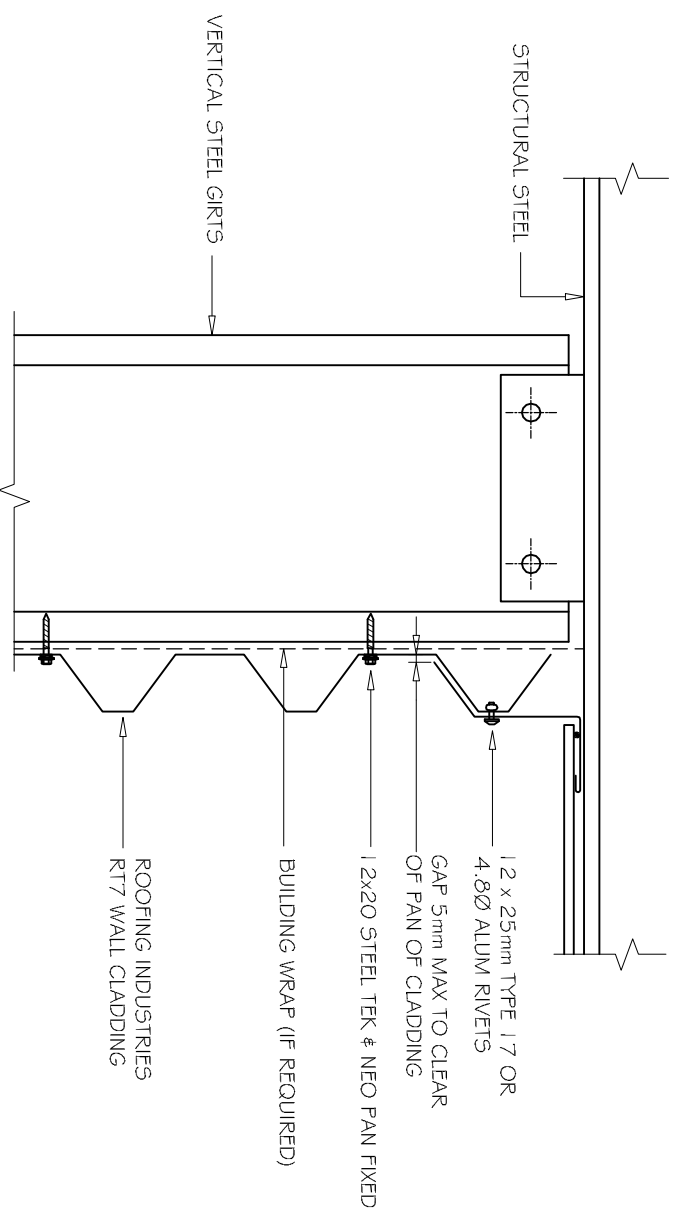
A HORIZONTAL RT7 HEAD DETAIL 1:5
