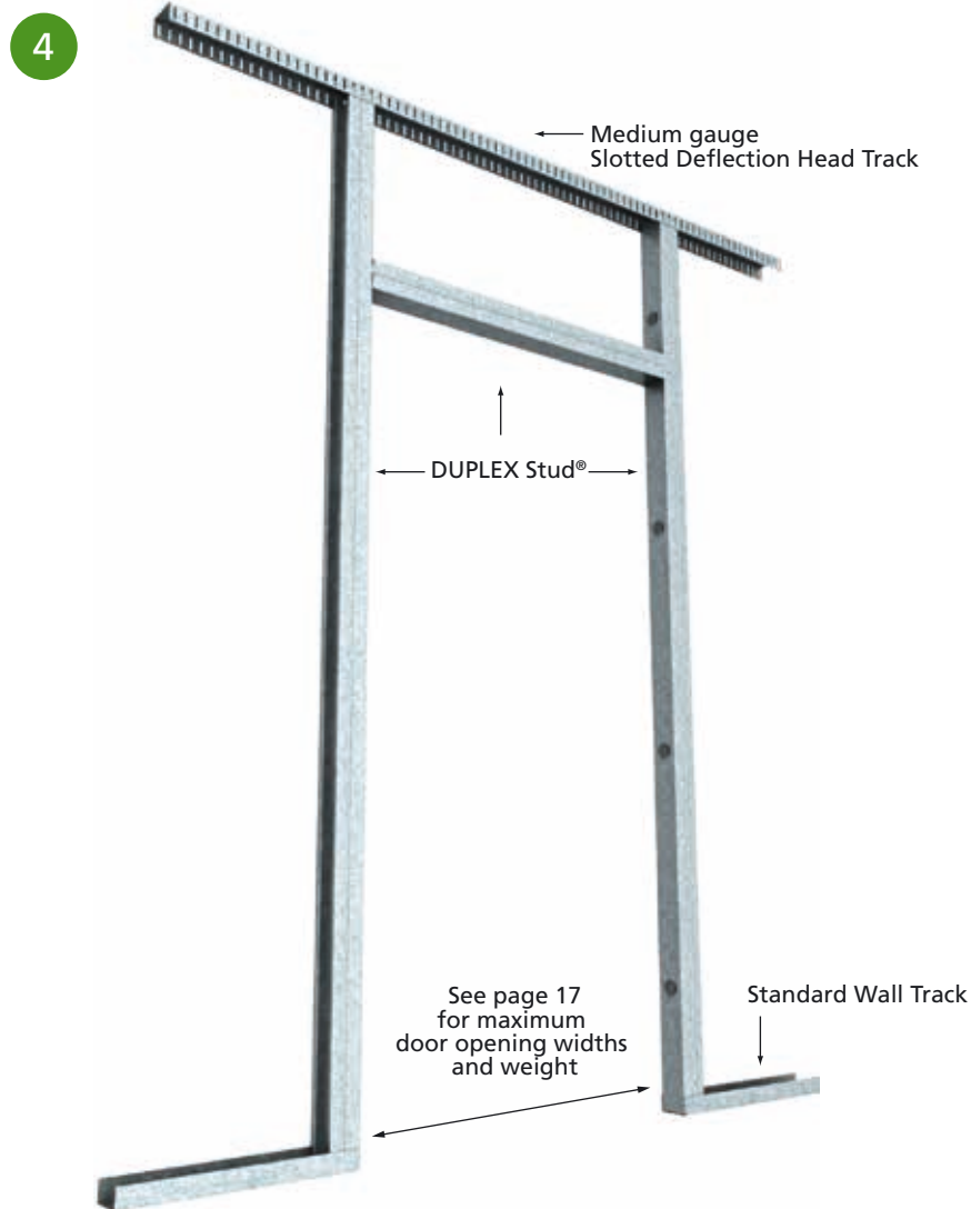
■ INTERNAL DOOR FRAMING: STANDARD OPENING
