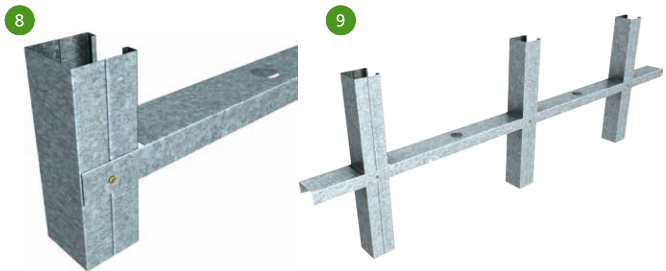
■ DOUBLE-PUNCHED NOGGING TRACK INSTALLATION
