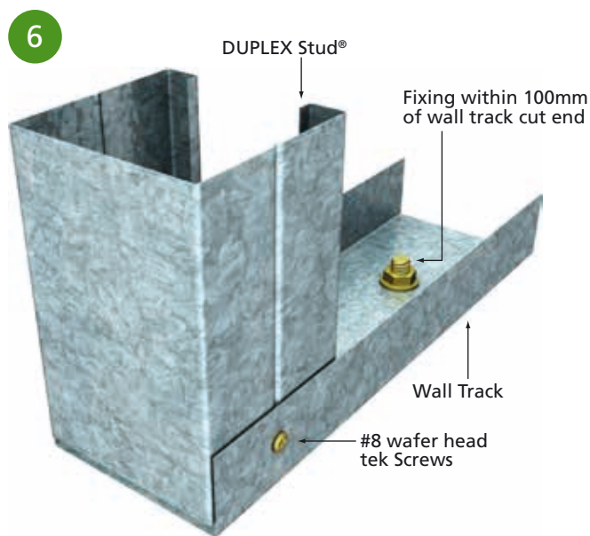
■ BASE WALL TRACK
