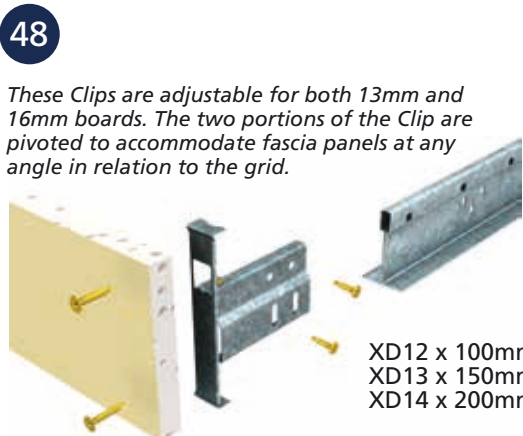
■ FASCIA TRIM CLIPS & TYPICAL APPLICATION
