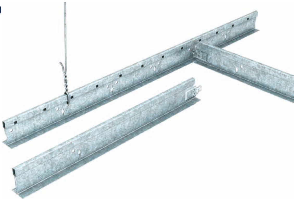
■ TYPICAL APPLICATION: OFF-MODULE GRID ARRANGEMENT (SEE ALSO FIGURE 11 ON PAGE 13)
