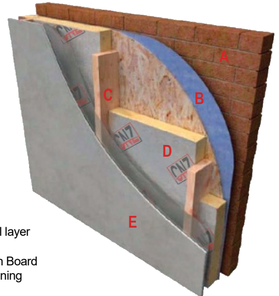
Figure 3.1. Fixing between studs
