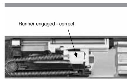
FIG 1a - Runner Engaged
