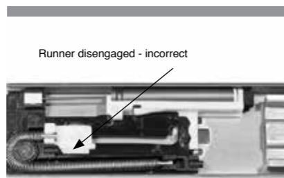
FIG 1b - Runner Disengaged
