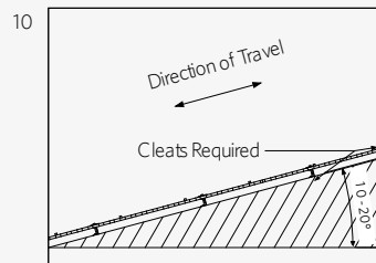
Walkway on Sloping Roofs (Along Slope) Walkway can be used in the range from 0° - 20°. Any walkway slope from 10° - 20° will need cleats installed. Cleat Spacings: Slopes 1 0° - 1 5° - 450mm Slopes 1 5° - 1 8° - 400mm Slopes 1 8° - 2 0° - 350mm
