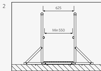
Width Between Guardrails Distance between guardrails, intermediate rails or toe boards shall not be less than 550mm Minimum width of walkway must be 600mm
