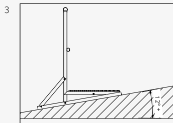
Guardrail on Sloping Roofs (Across Slope) Guardrail is required if the area adjacent to the walking area is 12° or greater.
