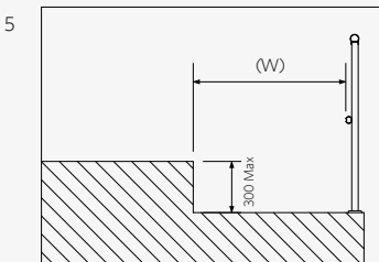
Guardrail on Platforms Height of Guardrail to be as follows Where width (W) is not less than 1 000mm, height shall be min 900mm. Where width (W) is less than 1 000mm, height shall be increased by 300mm.
