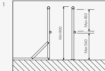
Guardrail Height Minimum height for guardrailing is 900mm from the walking surface.
