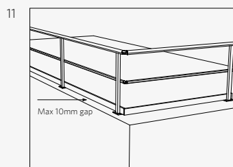
A toe board shall be installed on the edge of a platform or walkway where there is no permanent structure within 100mm of the edge and from which an object could fall to where persons have access to the area and to the side of a walkway. Maximum gap between the toe board and platform deck is 10mm.
