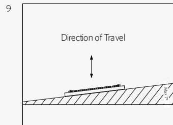
Walkway on Sloping Roofs (Across Slope) Maximum cross slope of walkway is 7° in the direction of travel. Preferred cross slope angle is 3°.
