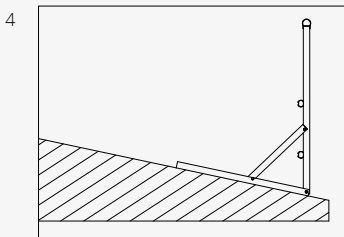
Guardrail on Sloping Roofs If there is guardrail on the edge of the roof where the slope is 12° or greater, a third rail is recommended.
