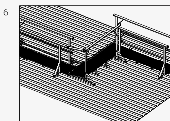
Walkway on Sloping Roofs (Along Slope) Walkways between 12° & 20 deg, a handrail shall be provided. Where there is a risk of a person rolling or sliding along the sloping surface of the walkway, the distance shall be limited to 1.8m (linear). A gate or change-in-direction is required if greater than 18 metres.
