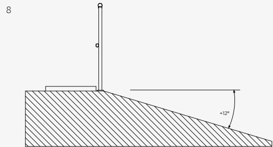
Guardrail is required if the angle of slope of the adjacent area to the walkway is more than 12° regardless of proximity to a fall edge.
