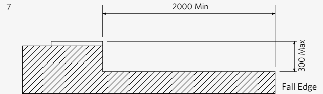
Guardrail is not required if the area adjacent to the walkway is not more than 300mm below the walking surface and is more than 2000mm from a fall edge.
