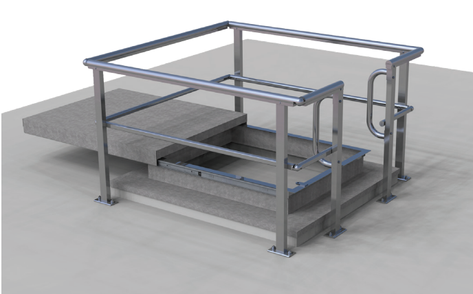
GW394C ACCESS HATCH GUARDRAIL KIT
