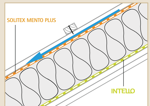
Fig. 58. A well protected roof structure
