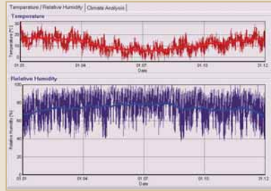
Fig. 40. Temperature and relative humidity
