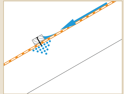
Fig. 57 a) & 57 b). Roof battens and protection against rain
