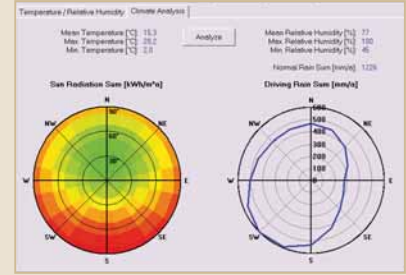
Fig. 37. Solar Radiation and Driving Rain
