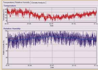
Fig. 36. Temperature and relative humidity
