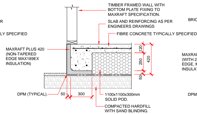
EXTERNAL FOOTING DETAIL 50mm STRAIGHT - 140mm FRAMING
