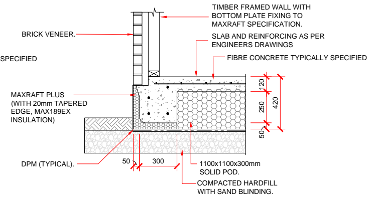
BRICK / STONE VENEER REBATE DETAIL
