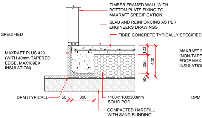
EXTERNAL FOOTING DETAIL 40mm TAPERED - 140mm FRAMING
