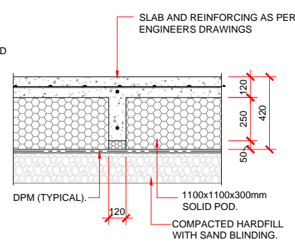
INTERNAL RIB DETAIL
