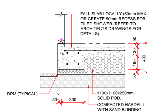
SHOWER RECESS DETAIL - 90mm FRAMING.
