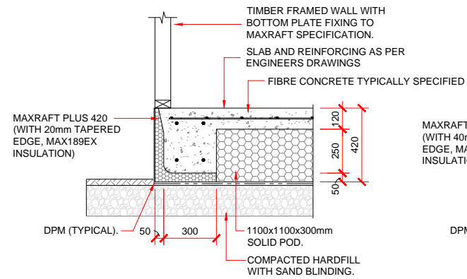
EXTERNAL FOOTING DETAIL 20mm TAPERED - 90mm/140mm FRAMING
