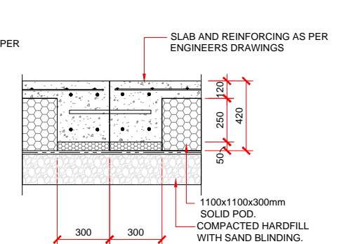
FREE JOINT / CONTROL JOINT DETAIL
