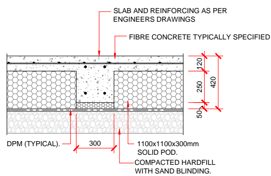
INTERNAL FOOTING DETAIL
