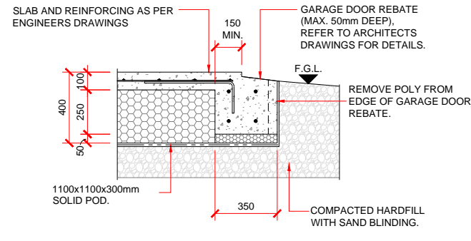
GARAGE DOOR REBATE DETAIL
