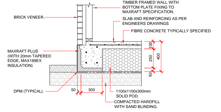
BRICK / STONE VENEER REBATE DETAIL
