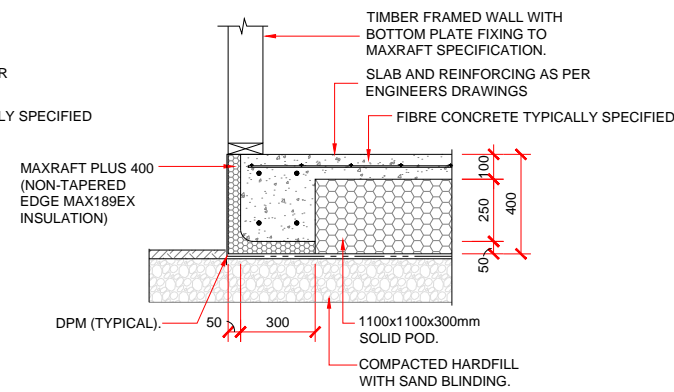
EXTERNAL FOOTING DETAIL 50mm STRAIGHT - 140mm FRAMING
