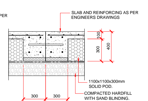
FREE JOINT / CONTROL JOINT DETAIL
