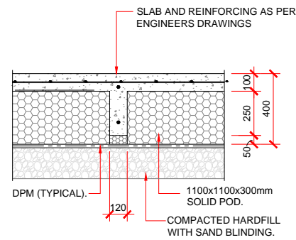
INTERNAL RIB DETAIL
