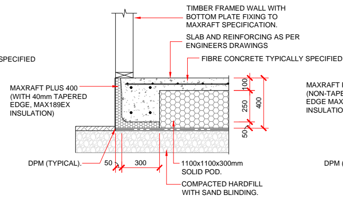
EXTERNAL FOOTING DETAIL 40mm TAPERED - 140mm FRAMING
