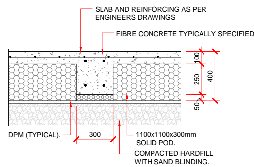
INTERNAL FOOTING DETAIL
