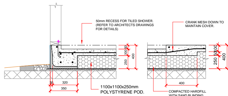
SHOWER RECESS DETAIL - 140mm FRAMING.
