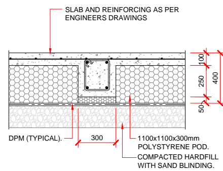
INTERNAL FOOTING DETAIL
