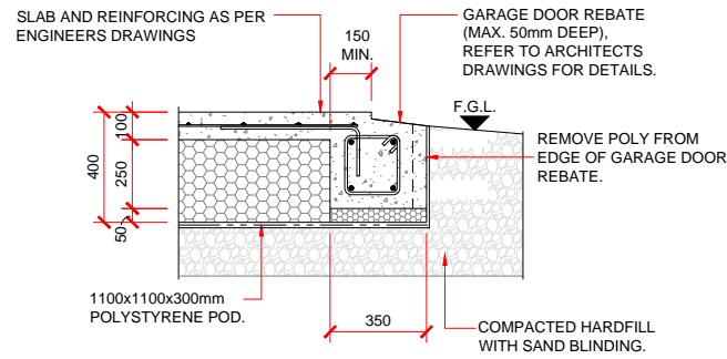
GARAGE DOOR REBATE DETAIL
