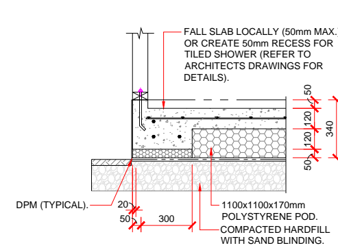
SHOWER RECESS DETAIL - 90mm FRAMING.
