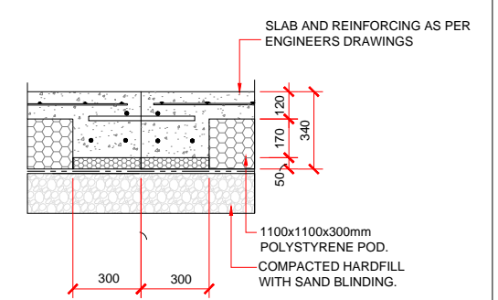
FREE JOINT / CONTROL JOINT DETAIL
