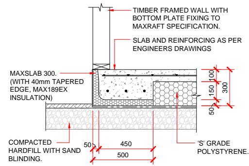
EXTERNAL FOOTING DETAIL 40mm TAPERED - 140mm FRAMING
