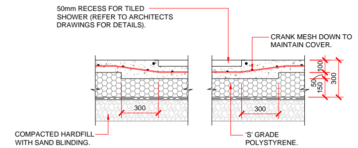
SHOWER RECESS DETAIL.
