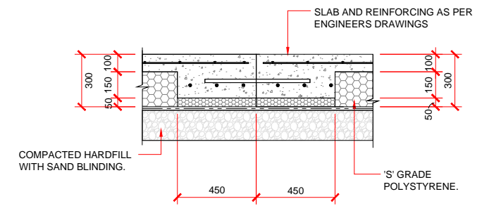
FREE JOINT / CONTROL JOINT DETAIL
