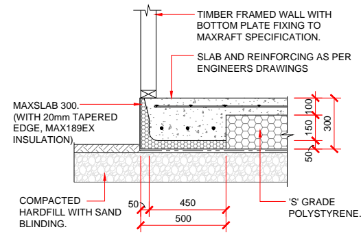
EXTERNAL FOOTING DETAIL 20mm TAPERED - 90mm/140mm FRAMING
