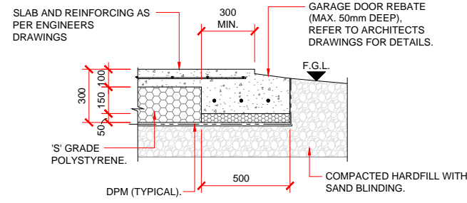
GARAGE DOOR REBATE DETAIL
