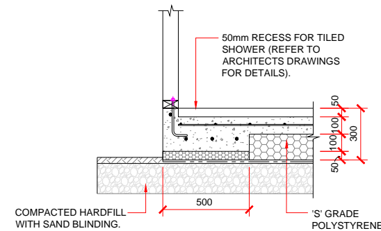
SHOWER RECESS DETAIL - 90mm FRAMING.
