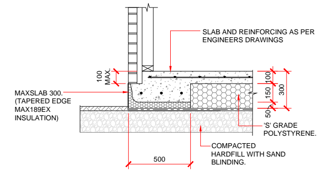
BRICK / STONE VENEER REBATE DETAIL
