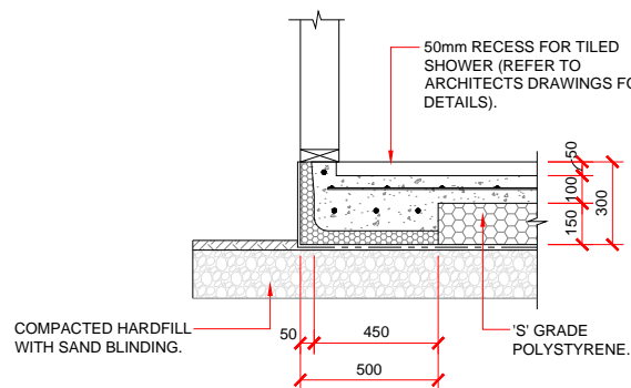
SHOWER RECESS DETAIL - 140mm FRAMING.
