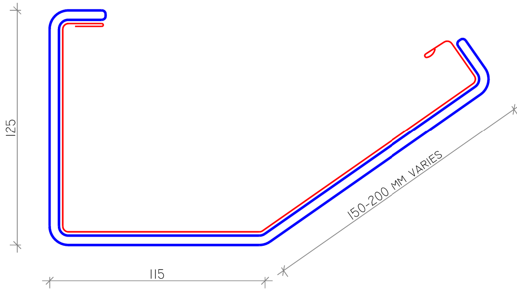
406mm CUSTOM GUTTER TYPE A
