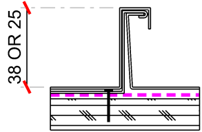
OVERLAPPING OF SEAMS BEFORE CRIMPING
