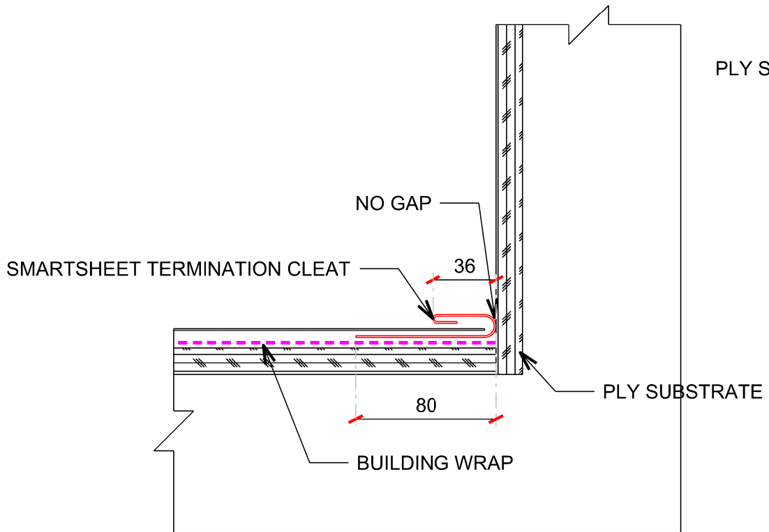
TERMINATION CLEAT
