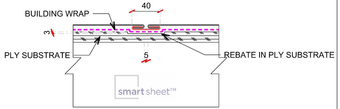
NEGATIVE JOINT
