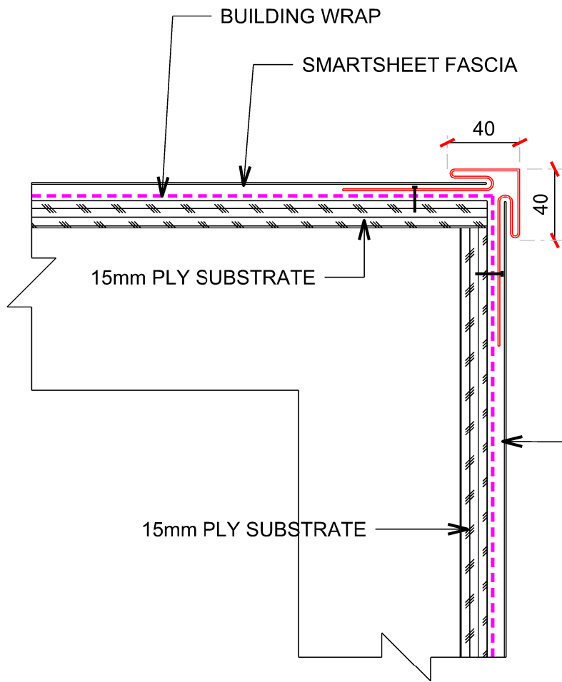
POSITIVE EXTERNAL CORNER
