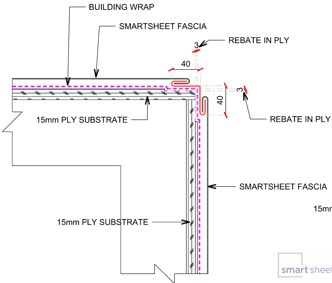
NEGATIVE EXTERNAL CORNER
