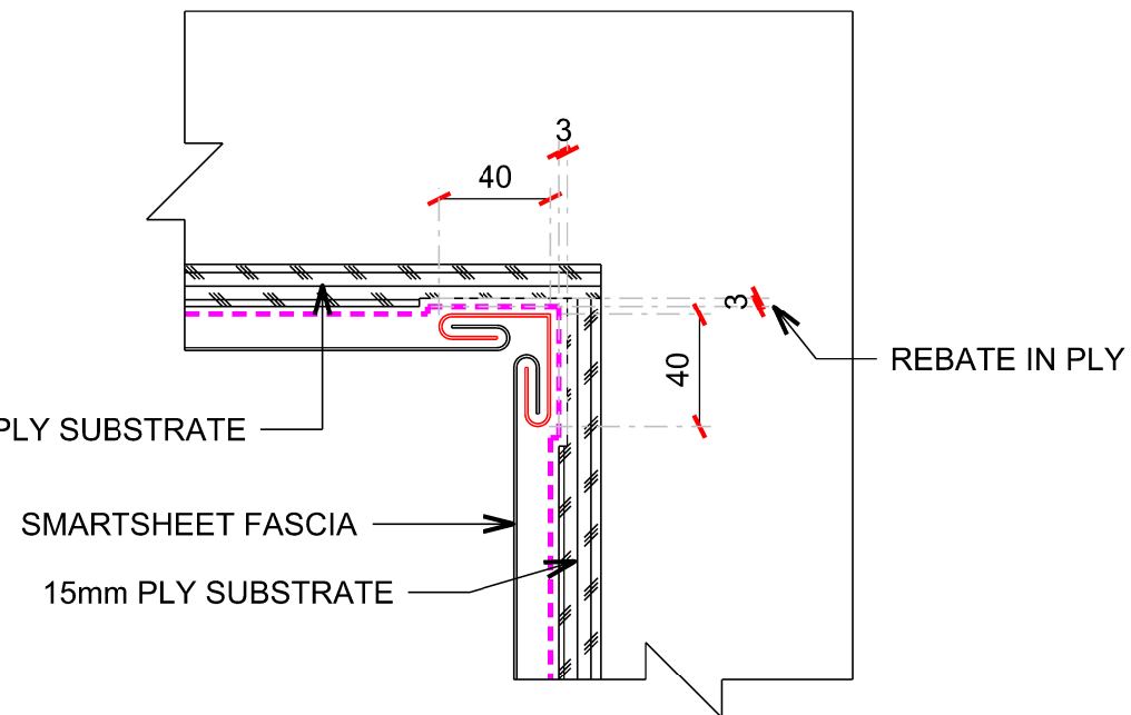
NEGATIVE INTERNAL CORNER
