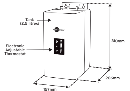
Easy to install under sink tank & water filter
