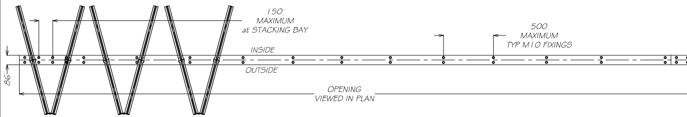
1 TYPICAL SYSTEMS SCHEMATICS SCALE: NTS
