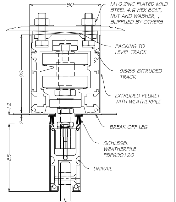
2 TOP RAIL SECTION SCALE: NTS
