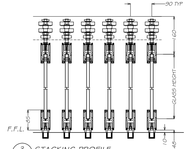
3 STACKING PROFILE SCALE: NTS
