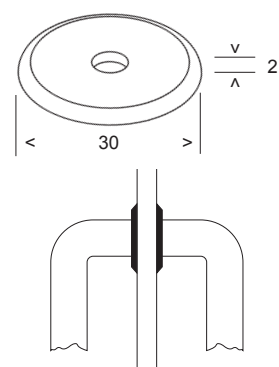
MW30 Highlight Washer To suit MK25 Knob Set and GT and M250 Handles
