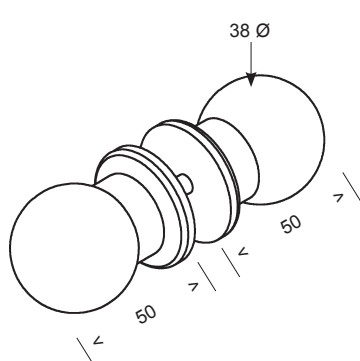
MK38 Pull Knob Set
