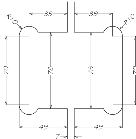
Glass to Glass Cut Out
