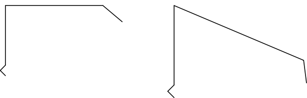
ROOFING INDUSTRIES BARGE FLASHING
