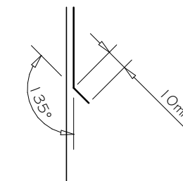
KICK-OUT at bottom edge of vertical flashing
