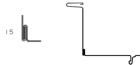
TWO PIECE FLASHING OPTION
