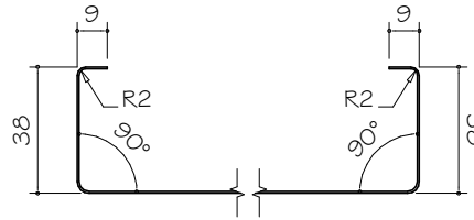
PROFILE PICTURED EX COIL PRIOR TO FOLDING. VARIABLE PAN WIDTH 206-706mm STANDARD WIDTH APPROX 515mm
