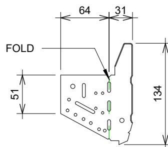
ROOFING INDUSTRIES 150 FASCIA BRACKET
