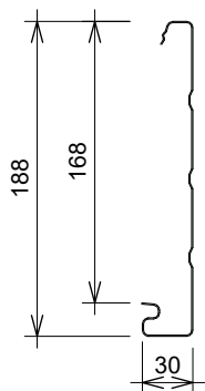
185 FASCIA COVER = 168mm
