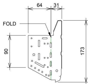
ROOFING INDUSTRIES 185 FASCIA BRACKET
