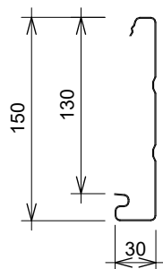
150 FASCIA COVER = 130mm
