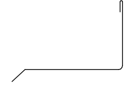
ROOFING INDUSTRIES APRON FLASHING
